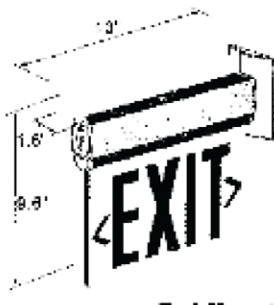
End Mounting
